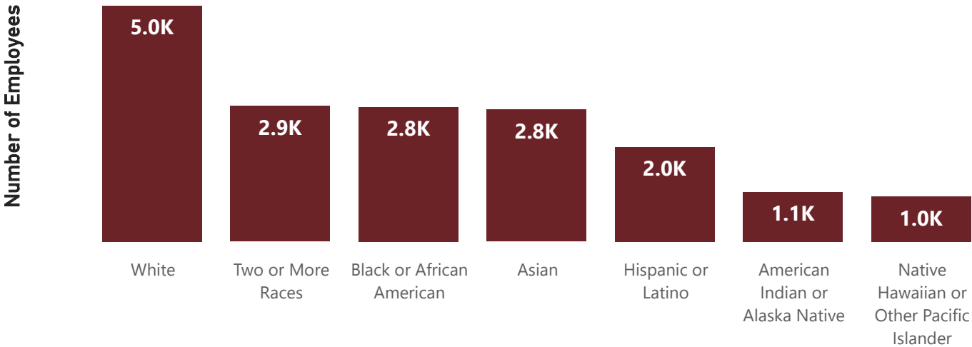
Race Distribution
